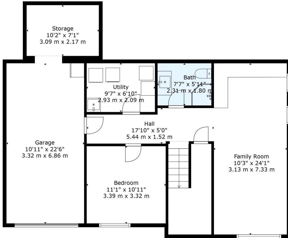
Floor 1
