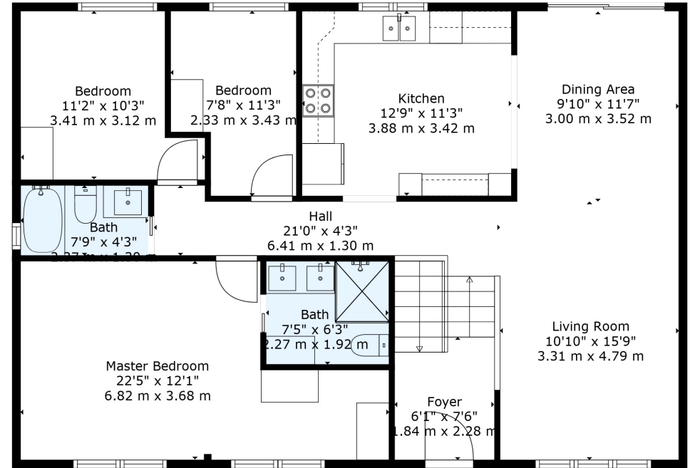
Floor 2
